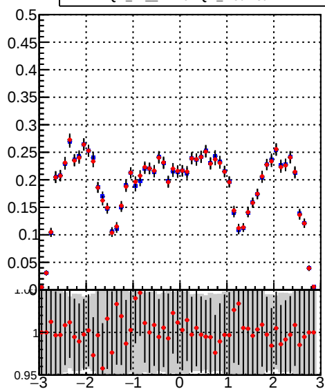
DQM_TT_mkFit-DQM_original DQM_TT_mkFit-DQM_modified
