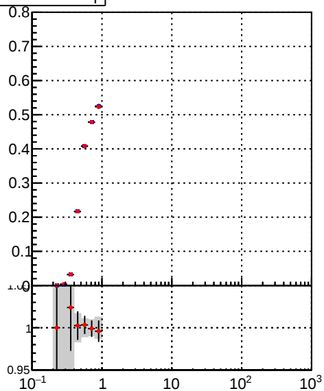
DQM_TT_mkFit-DQM_original DQM_TT_mkFit-DQM_modified
