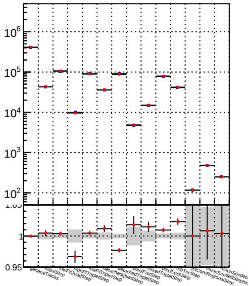
Number —●— DQM_TT__mkFit-DQM_modified
