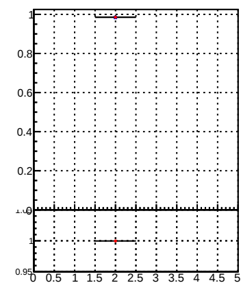
Fake rate vs hit Legend: DQM_TT_mkFit-DQM_original (blue line), DQM_TT_mkFit-DQM_modified (red line)
