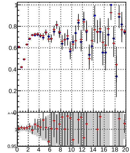
Fake rate vs. —●— DQM TT mkFit-DQM_original —●— DQM TT mkFit-DQM_modified
