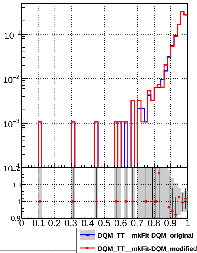
RecoPVAssoc2GenPVMatched_Missing
