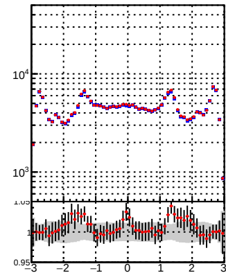
N of reco track vs \eta Legend: DQM_TT_mkFit-DQM_original (blue dots) DQM_TT_mkFit-DQM_modified (red dots)
