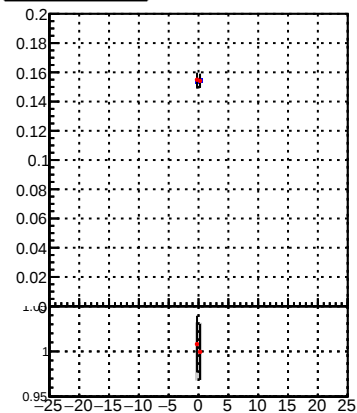
—●— DQM_TT_mkFit-DQM_original —●— DQM_TT_mkFit-DQM_modified
