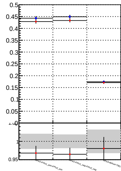
Fake rate vs. —●— DQM_TT_mkFit-DQM_original —●— DQM_TT_mkFit-DQM_modified
