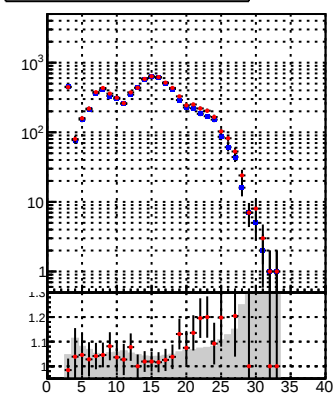
DQM_TT_mkFit-DQM_original DQM_TT_mkFit-DQM_modified
