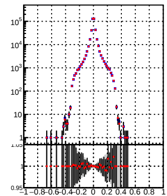
Legend: DQM_TT_mkFit-DQM_original (Black line with dots) DQM_TT_mkFit-DQM_modified (Red line with dots)
