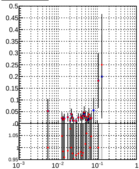
Fake rate vs dr DQM_TT_mkFit-DQM_original DQM_TT_mkFit-DQM_modified
