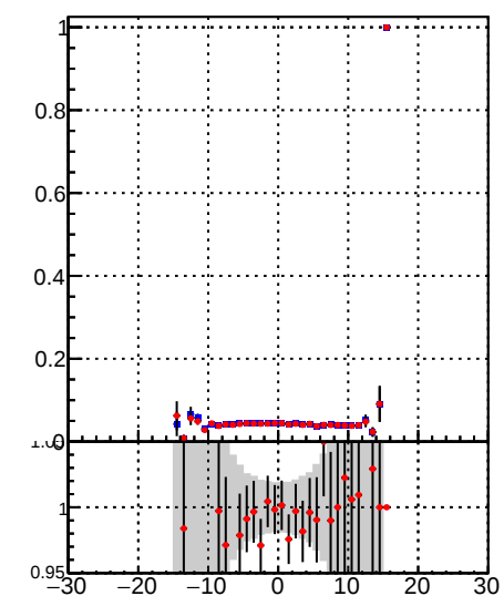
Fake rate vs d DQM TT mkFit-DQM_original DQM TT mkFit-DQM_modified
