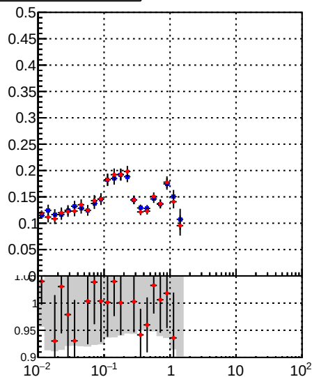
—•— DQM_TT_mkFit-DQM_original —•— DQM_TT_mkFit-DQM_modified
