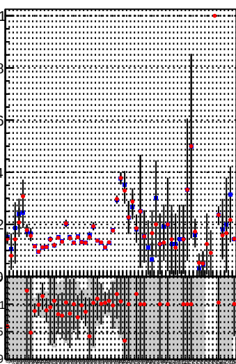
Fake rate vs. —●— DQM TT mkFit-DQM_original —●— DQM TT mkFit-DQM_modified
