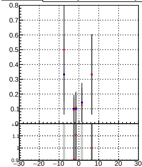
—•— DQM_TT_mkFit-DQM_original —•— DQM_TT_mkFit-DQM_modified
