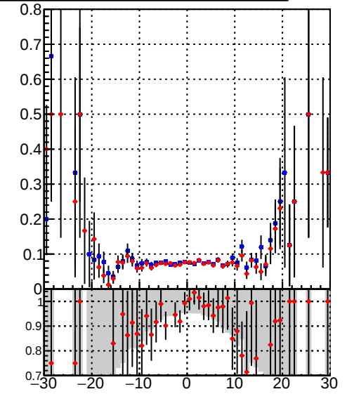
Efficiency vs vertpos Legend: — DQM_TT_mkFit-DQM_original — DQM_TT_mkFit-DQM_modified
