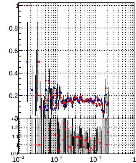
—•— DQM_TT_mkFit-DQM_original —•— DQM_TT_mkFit-DQM_modified
