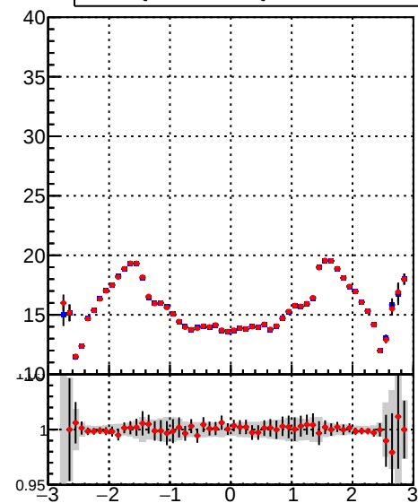
mean hit — DQM_TT_mkFit-DQM_original — DQM_TT_mkFit-DQM_modified
