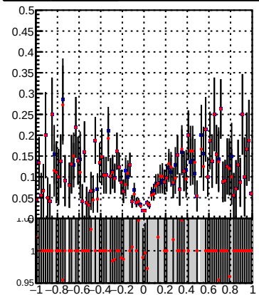
Efficiency —●— DQM_TT_mkFit-DQM_original —●— DQM_TT_mkFit-DQM_modified
