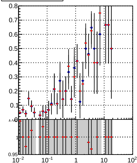
■ DQM_TT_mkFit-DQM_original ● DQM_TT_mkFit-DQM_modified
