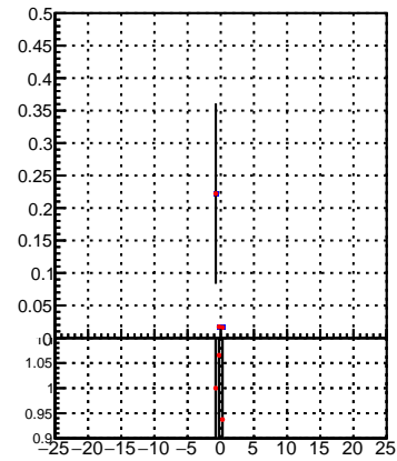
—●— DQM_TT_mkFit-DQM_original —●— DQM_TT_mkFit-DQM_modified
