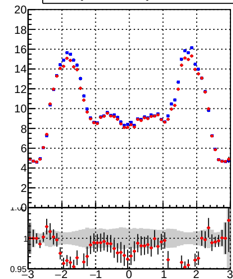
mean hit Legend: — DQM_TT_mkFit-DQM_original — DQM_TT_mkFit-DQM_modified
