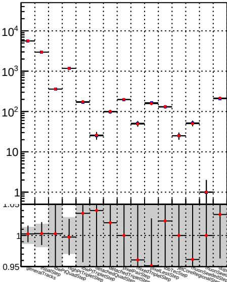
Number —●— DQM_TT__mkFit-DQM_modified
