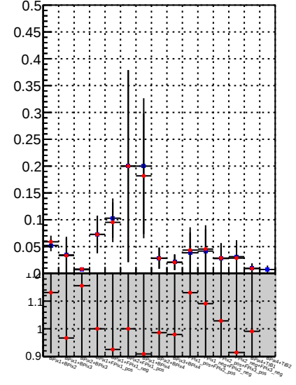
Fake rate vs. —●— DQM_TT_mkFit-DQM_original —●— DQM_TT_mkFit-DQM_modified
