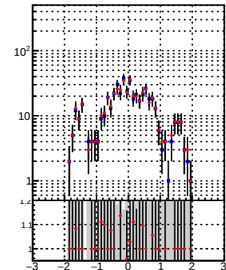
—•— DQM_TT_mkFit-DQM_original -.-.- DQM_TT_mkFit-DQM_modified
