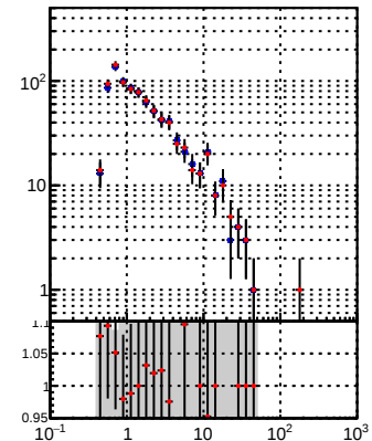
—•— DQM_TT_mkFit-DQM_original -.-.- DQM_TT_mkFit-DQM_modified
