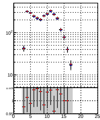
—●— DQM_TT_mkFit-QM_original —●— DQM_TT_mkFit-QM_modified
