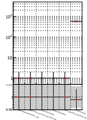
N of reco track vs. \chi^2
