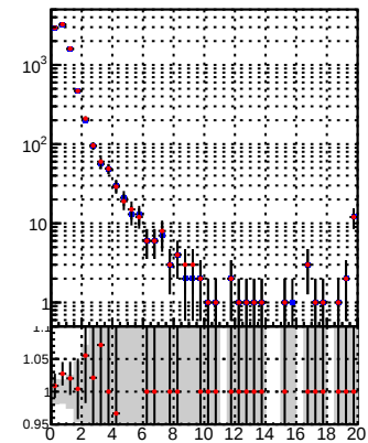
Legend: - DQM TT mkFit-DQM_original (blue circles) - DQM TT mkFit-DQM_modified (red circles)
