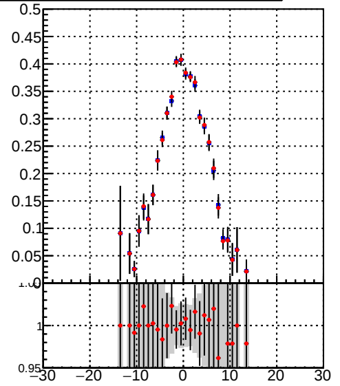
Efficiency vs. sim PV z — DQM_TT_mkFit-DQM_original — DQM_TT_mkFit-DQM_modified
