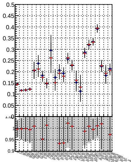
Fake rate vs. DQM_TT_mkFit-DQM_original DQM_TT_mkFit-DQM_modified
