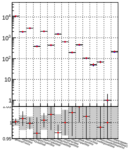
Number —●— DQM_TT__mkFit-DQM_modified
