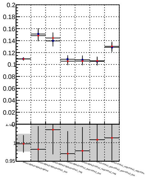
Fake rate vs. —●— DQM_TT_mkFit-DQM_original —●— DQM_TT_mkFit-DQM_modified
