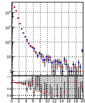
N of reco track vs. \chi^2 — DQM TT mkFit-DQM_original — DQM TT mkFit-DQM_modified
