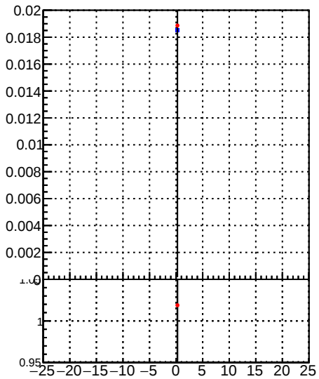
Fake rate vs d —●— DQM_TT_mkFit-DQM_original —●— DQM_TT_mkFit-DQM_modified
