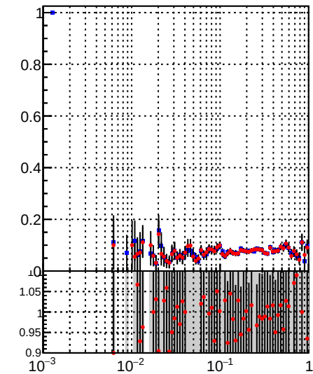
Fake rate vs \sqrt{s} DQM_TT_mkFit-DQM_original DQM_TT_mkFit-DQM_modified
