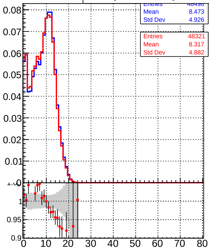
—■— DQM_TT_mkFit-DQM_original —●— DQM_TT_mkFit-DQM_modified
