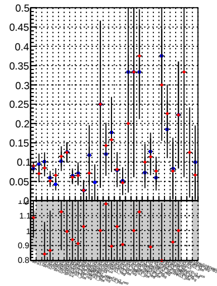
Fake rate vs. \chi^2
