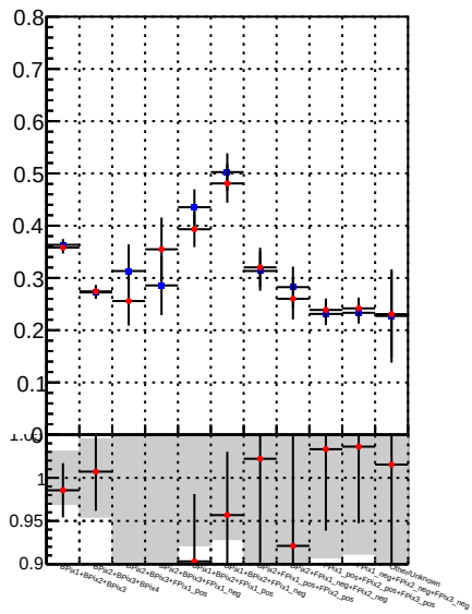
Fake rate vs. —●— DQM TT mkFit-DQM_original —●— DQM TT mkFit-DQM_modified
