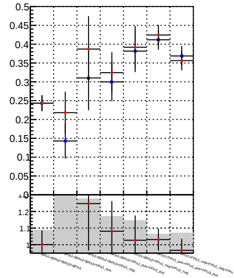
Fake rate vs. —•— DQM_TT_mkFit-DQM_original —•— DQM_TT_mkFit-DQM_modified
