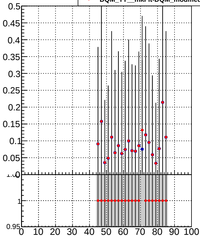
■ DQM_TT_mkFit-DQM_original ● DQM_TT_mkFit-DQM_modified
