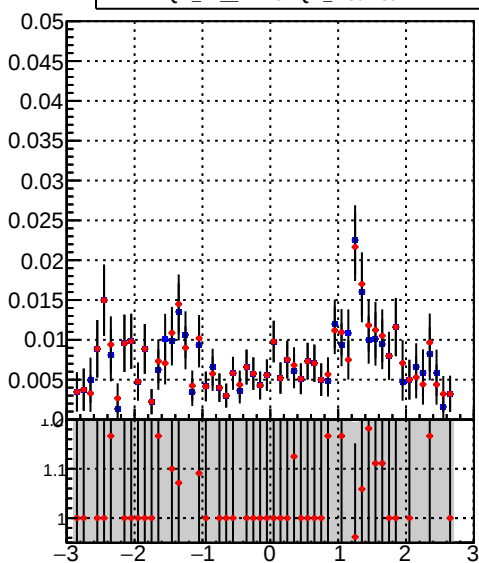
—●— DQM_TT_mkFit-DQM_original —●— DQM_TT_mkFit-DQM_modified
