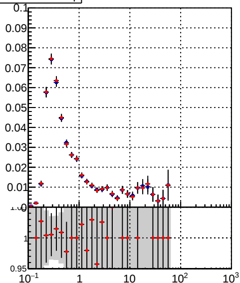
—●— DQM_TT_mkFit-DQM_original —●— DQM_TT_mkFit-DQM_modified
