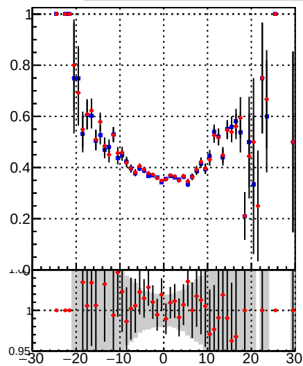
—•— DQM_TT_mkFit-DQM_original —•— DQM_TT_mkFit-DQM_modified
