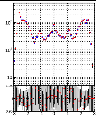
—●— DQM_TT_mkFit-DQM_original —●— DQM_TT_mkFit-DQM_modified
