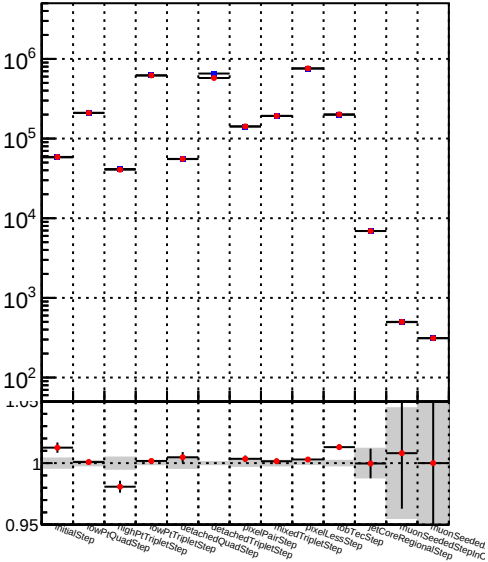
Number —●— DQM_TT__mkFit-DQM_modified
