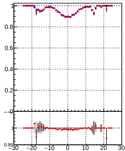
—•— DQM_TT_mkFit-DQM_original —•— DQM_TT_mkFit-DQM_modified
