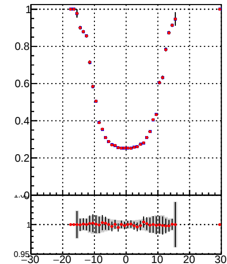
—•— DQM_TT_mkFit-DQM_original —•— DQM_TT_mkFit-DQM_modified
