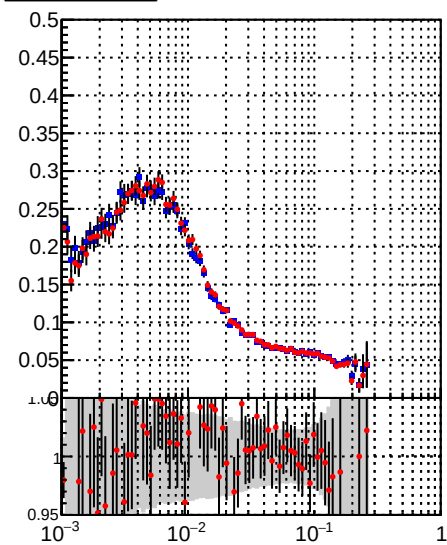
—●— DQM_TT_mkFit-DQM_original —●— DQM_TT_mkFit-DQM_modified
