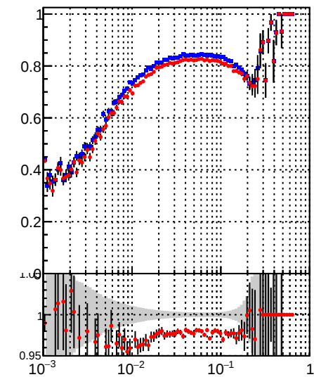
—●— DQM_TT_mkFit-QM_original —●— DQM_TT_mkFit-QM_modified
