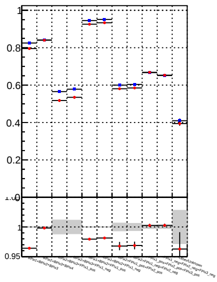
Fake rate vs. —●— DQM_TT_mkFit-DQM_original —●— DQM_TT_mkFit-DQM_modified
