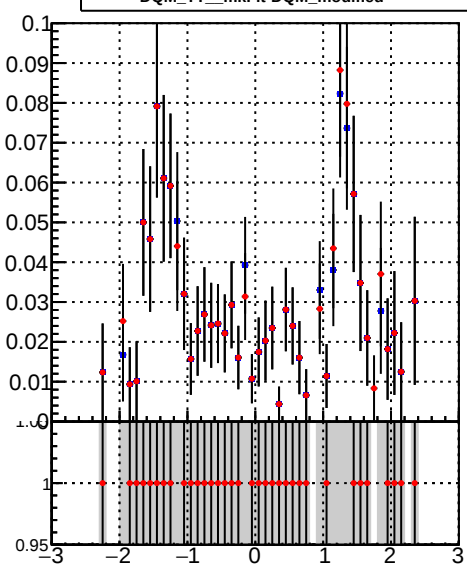
—●— DQM_TT_mkFit-DQM_original —●— DQM_TT_mkFit-DQM_modified
